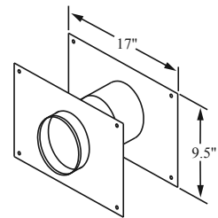
Wall Thimble Part No. 6911109
