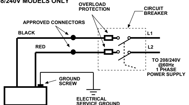
FIGURE 5 WIRING DIAGRAM 208/240V MODELS ONLY
