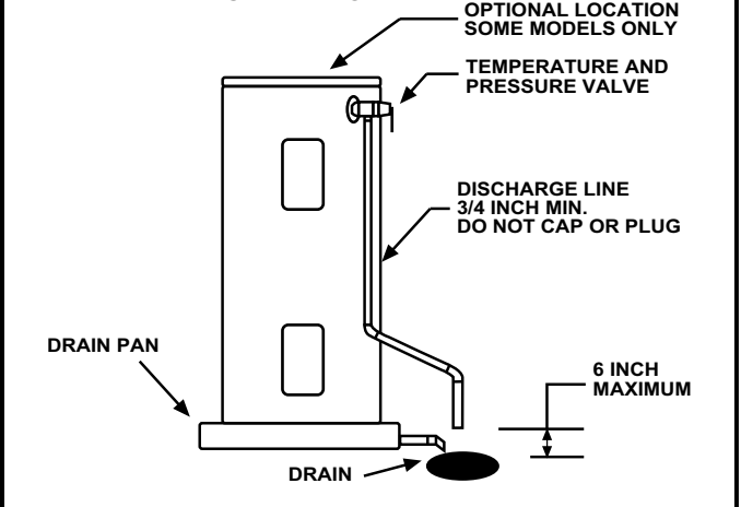
FIGURE 9 TEMPERATURE AND PRESSURE RELIEF VALVE INSTALLATION
