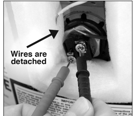
Figure 24 - Use a multimeter to check the resistance of the upper heating element.
