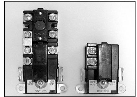
Figure 38 - Upper and Lower Thermostats
