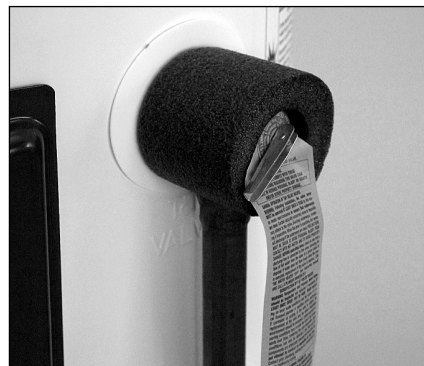
Figure 14 - Make sure the insulation does not interfere with the T&P Relief Valve's operation.
