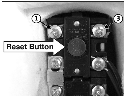
Figure 25 - Energy Cut Off (ECO) button
