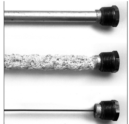
Figure 29 - Anode Rods from new (top) to partially depleted (middle) to fully depleted staged (bottom)
