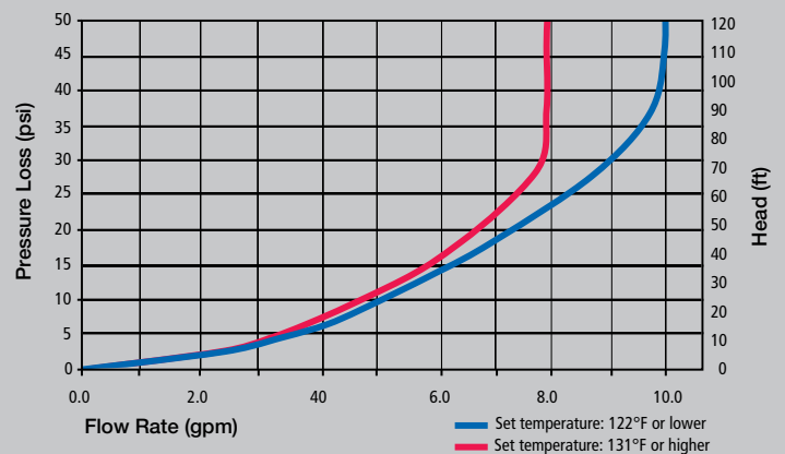
510: Pressure Loss
