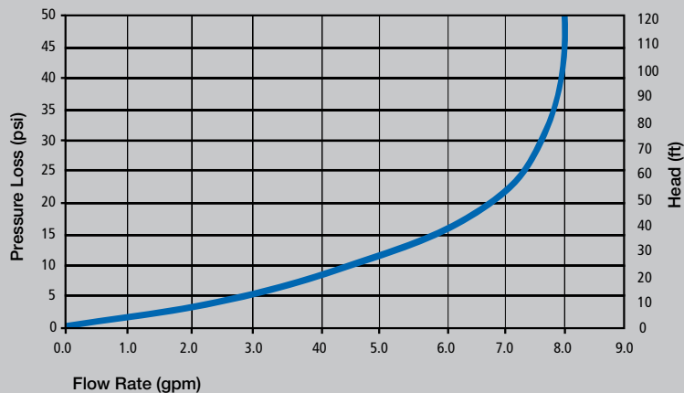
310: Pressure Loss
