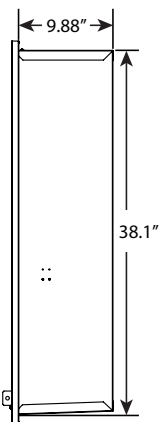
Recess Box for Retrofit: 100266729
