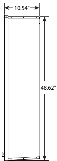
Recess Box for Retrofit: 100298009
