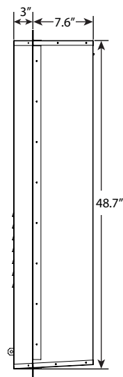
Recess Box for New Construction: 100306285
