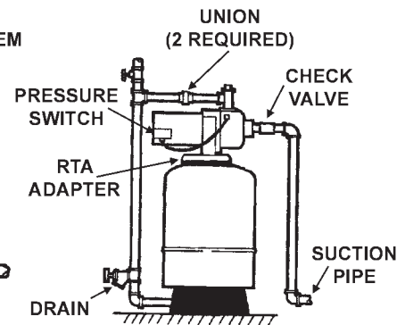
JET PUMP MOUNTED ON VERTICAL TANK
