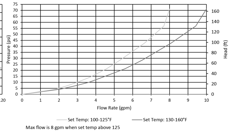
540H3 PRESSURE LOSS
