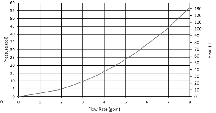
340H3 PRESSURE LOSS
