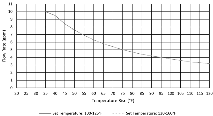
540H3 OUTPUT TEMP VS. GPM
