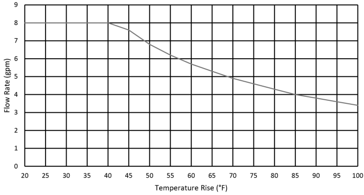
340H3 OUTPUT TEMP VS. GPM
